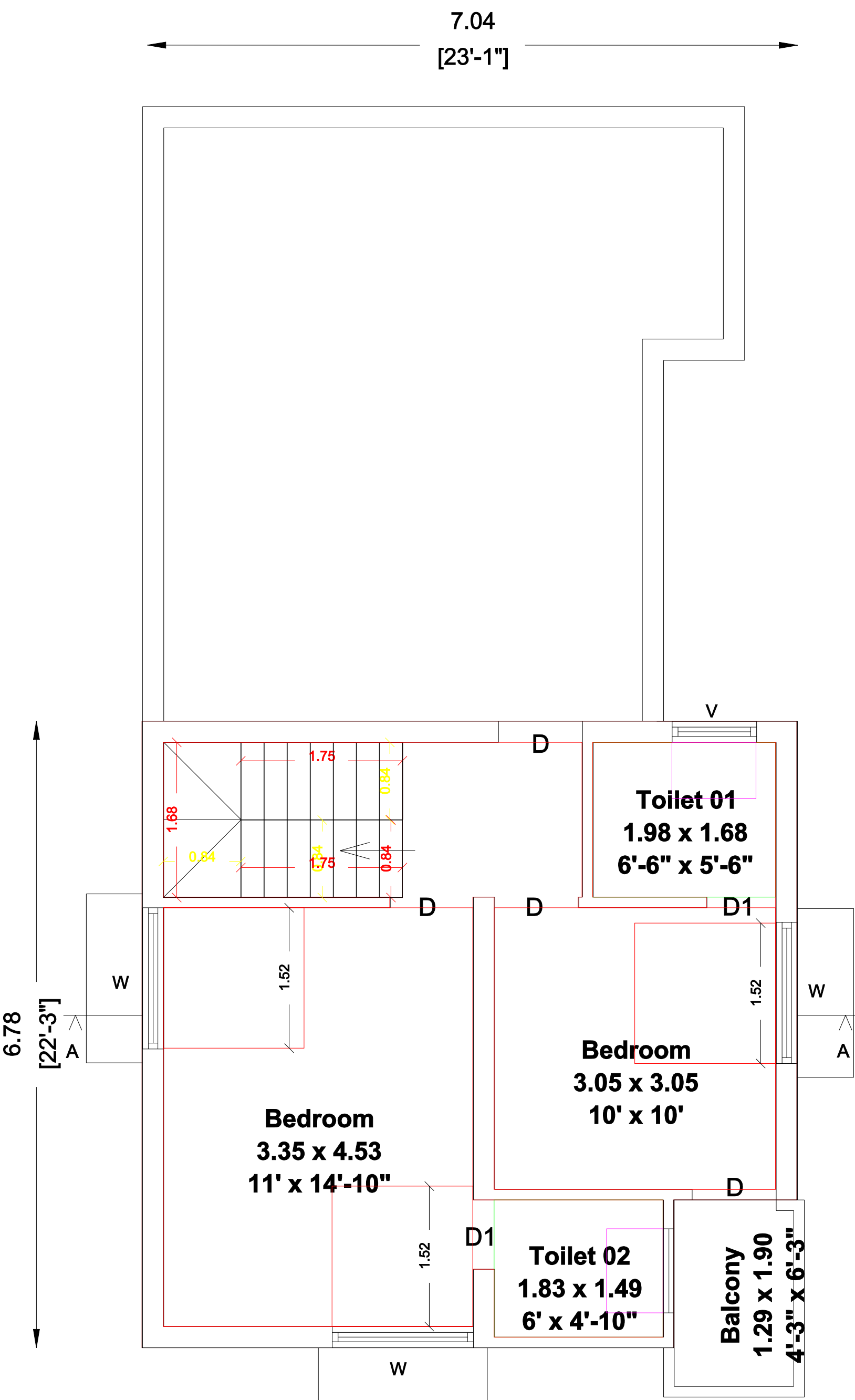
PRO. FIRST FLOOR PLAN
