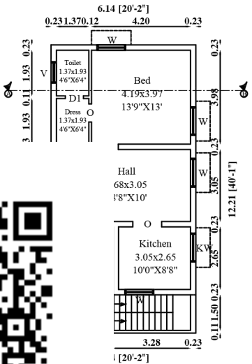
Floor Plan
