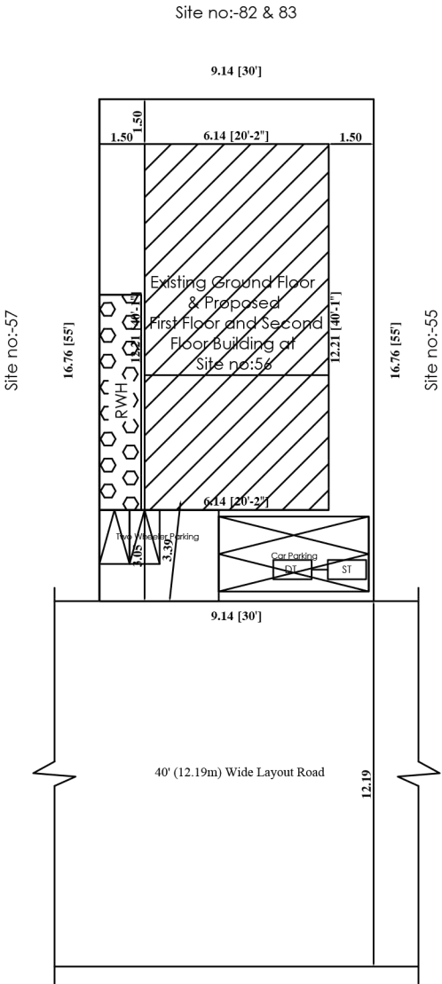
Site Plan
