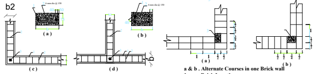
Figure - 2 : Typical Details of Providing Vertical Steel bars in Brick Masonry.
