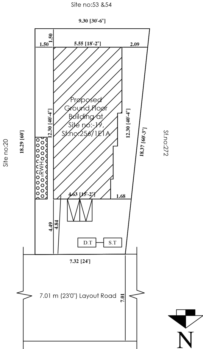
Site Plan
