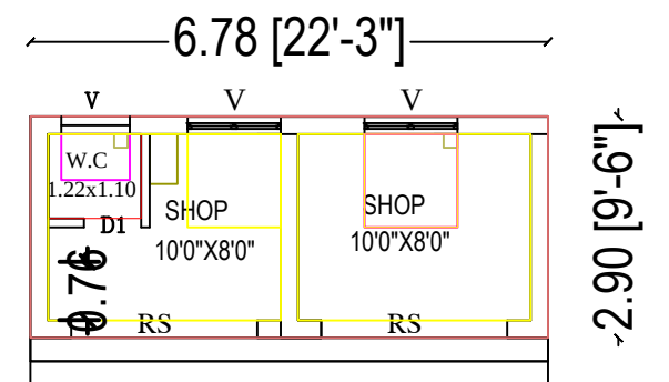
PROPOSED SHOP PLAN
