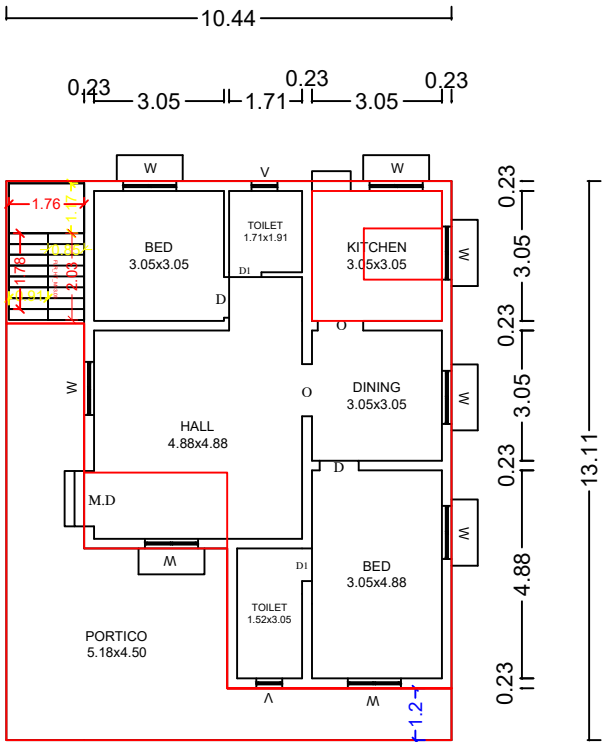
EX.GROUND FLOOR
