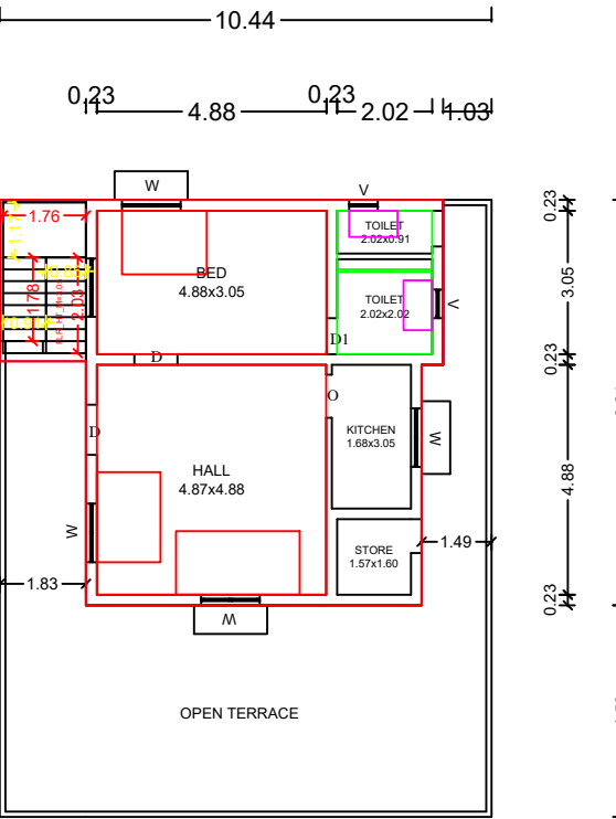
PRO.ADD.SECOND FLOOR
