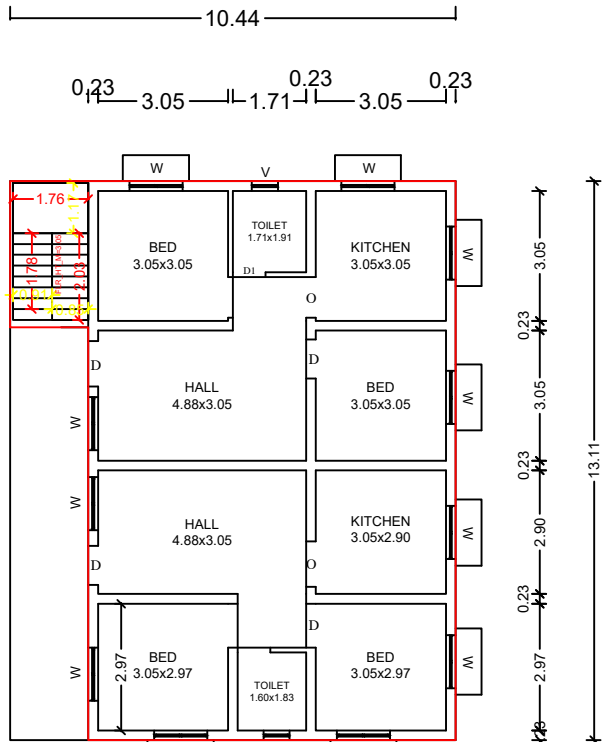
EX.FIRST FLOOR
