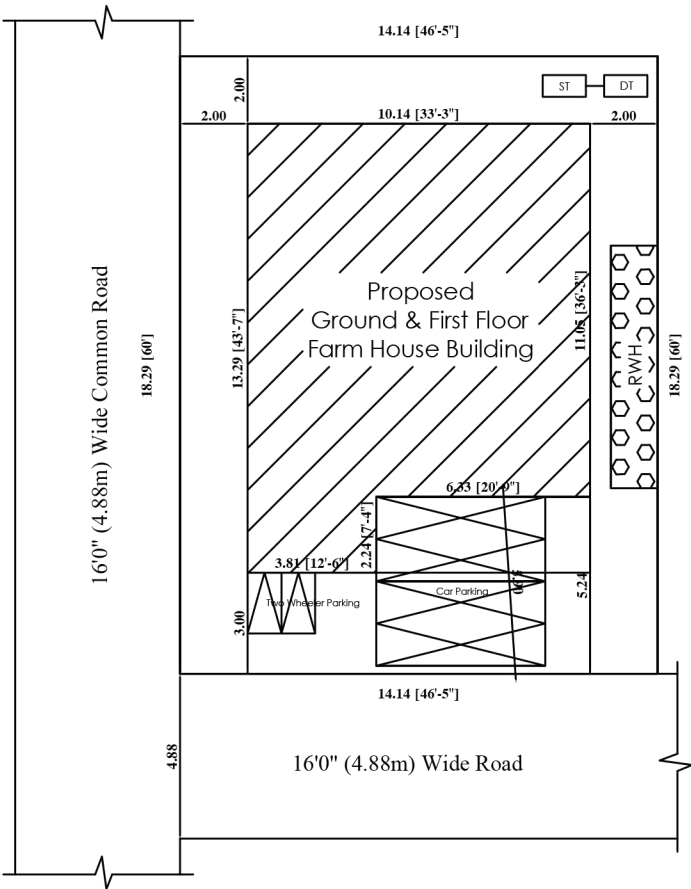
Site Plan
