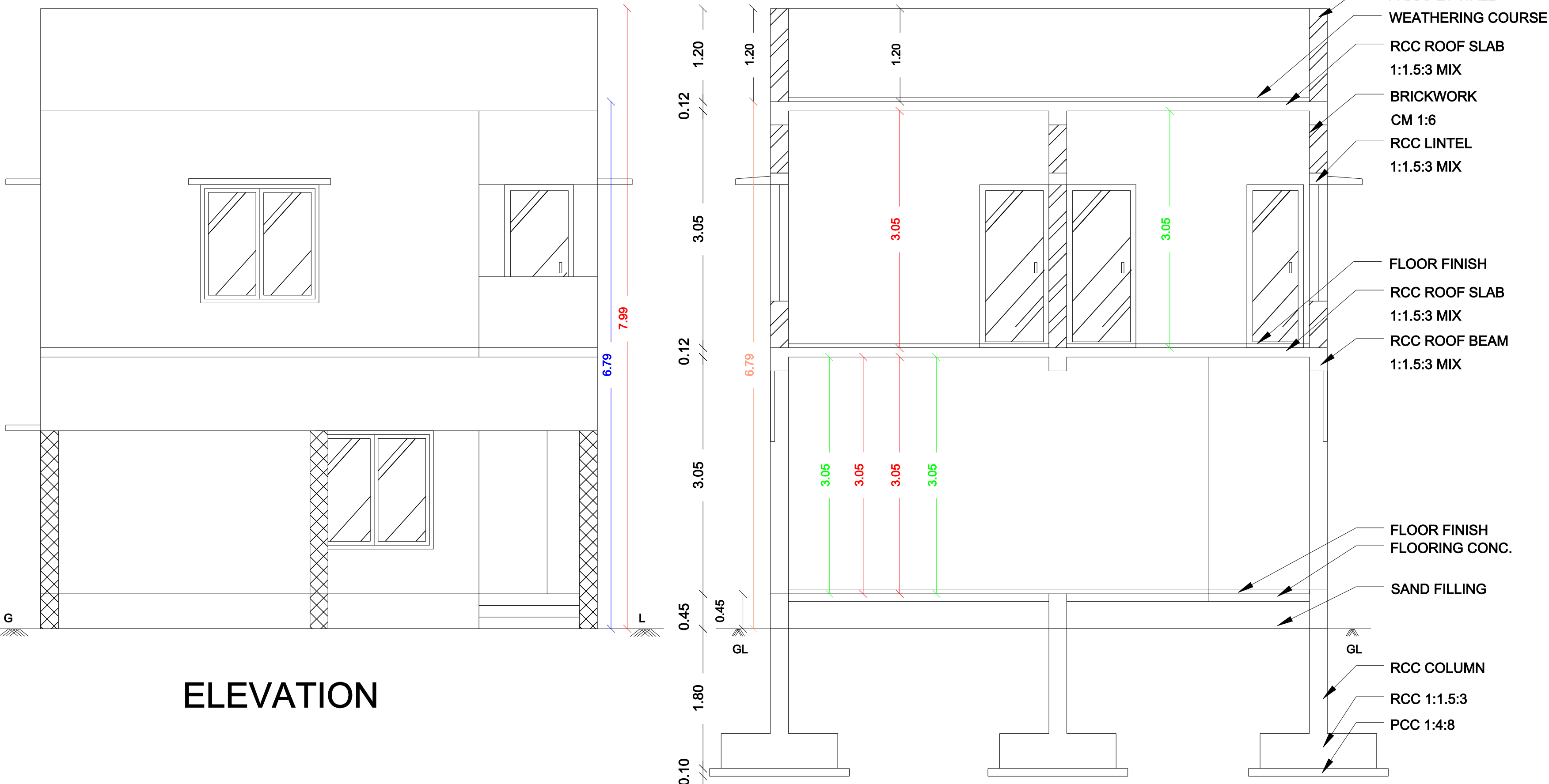
SECTION-AA
