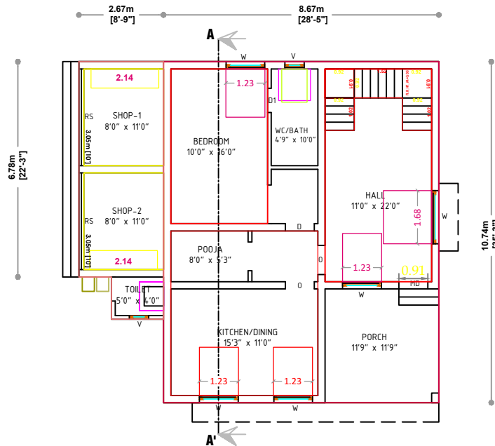
PROPOSED GROUND FLOOR PLAN (EAST FACING)
