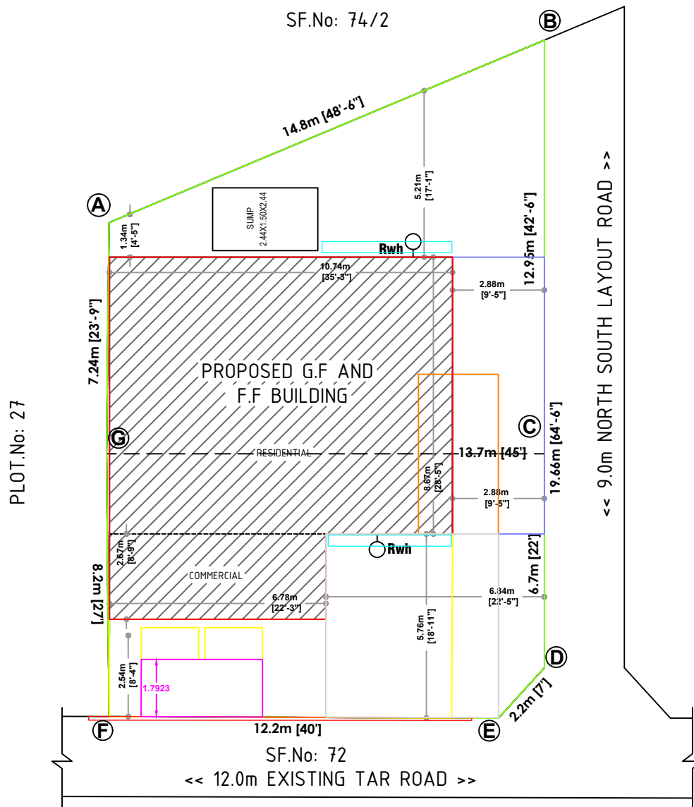
SITE PLAN
