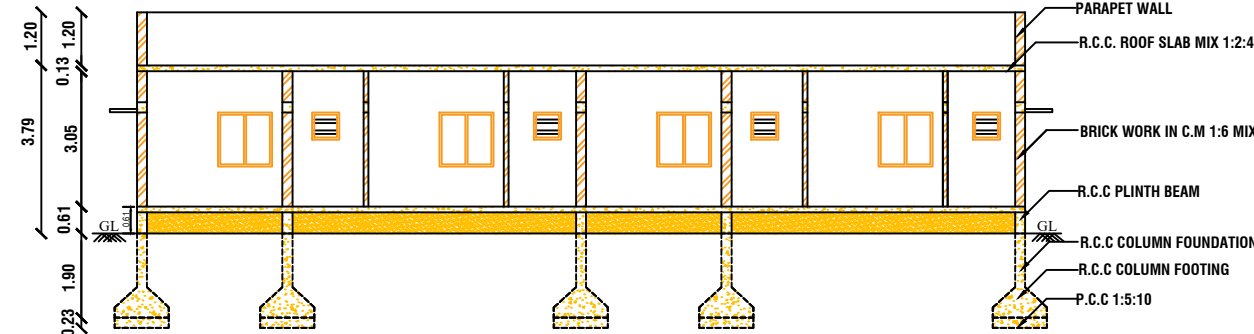
CROSS SECTION AT A-A
