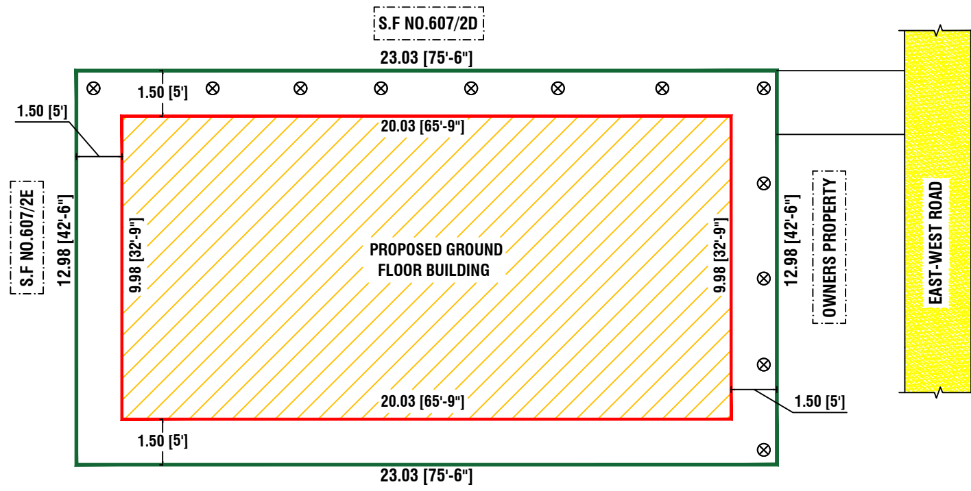
SITE PLAN
