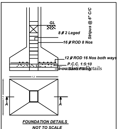
FOUNDATION DETAILS (NOT TO SCALE)
