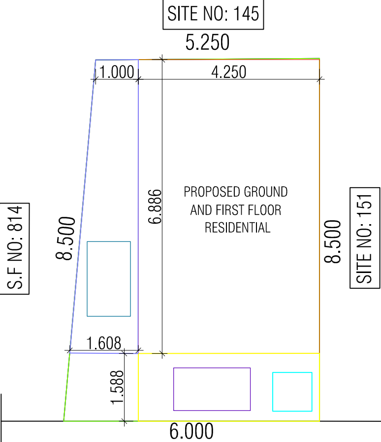
KEY PLAN
