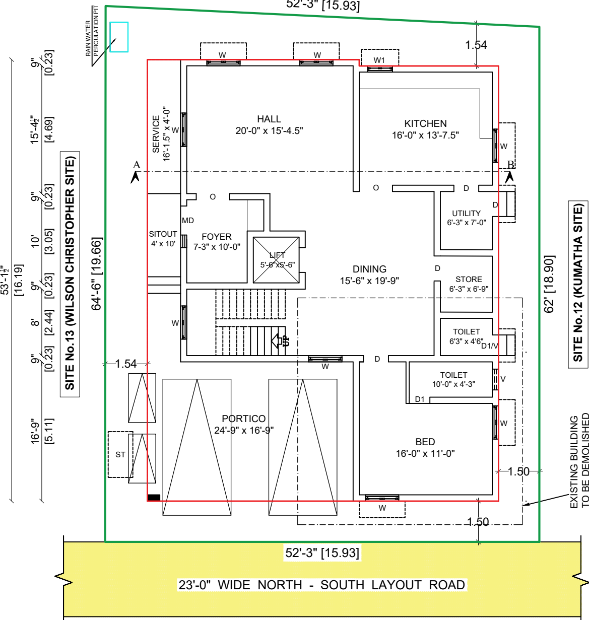
SITE CUM GROUND FLOOR PLAN
