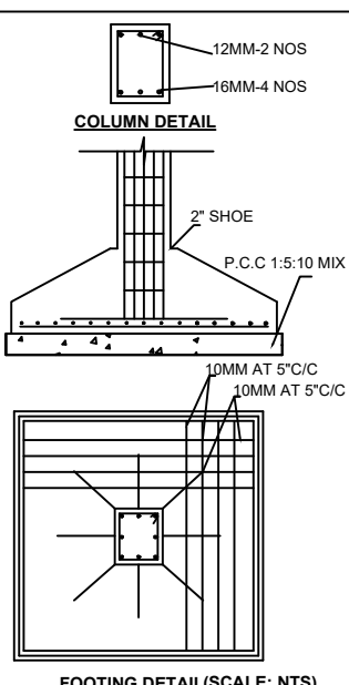
FOOTING DETAIL(SCALE: NTS)
