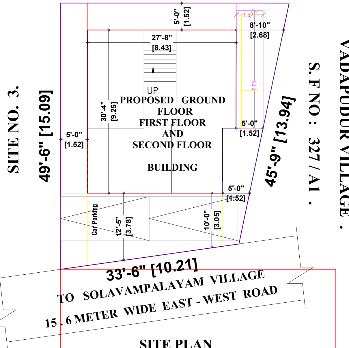
SITE PLAN
