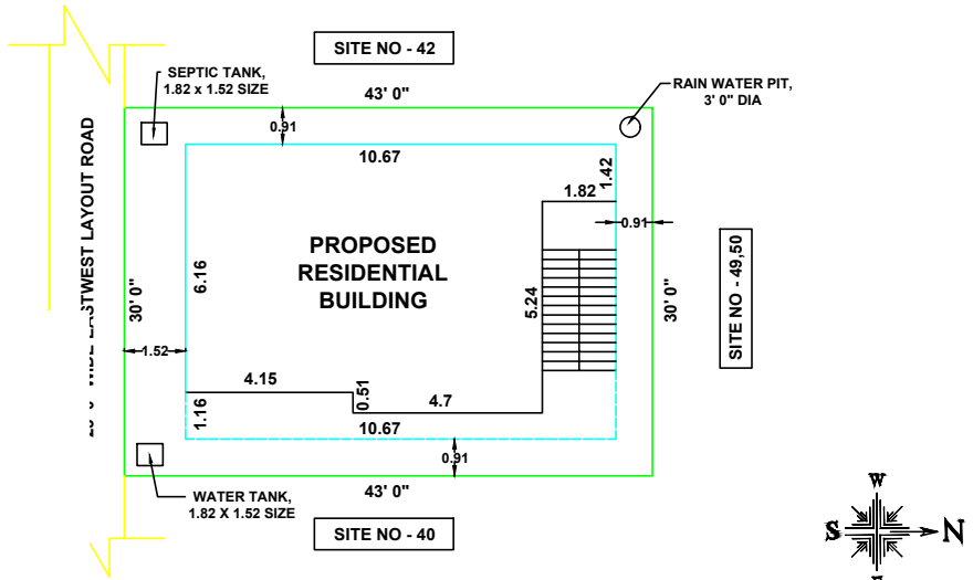
SITE PLAN SCALE - 1' 0" = 10' 0"
