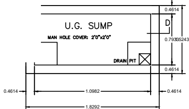
SUMP DETAIL SCALE 1" - 4'0"
