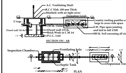
SEPTIC TANK WITH DISPERSION TRENCH (250 Gls.)
