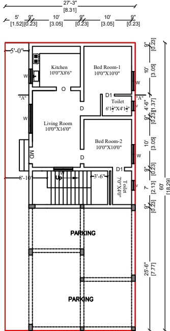
PRO. GROUND FLOOR PLAN
