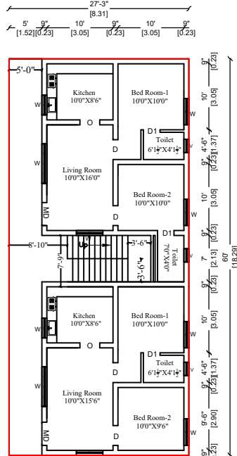
PRO. FIRST FLOOR PLAN
