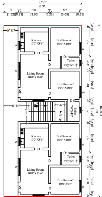
PRO. SECOND FLOOR PLAN
