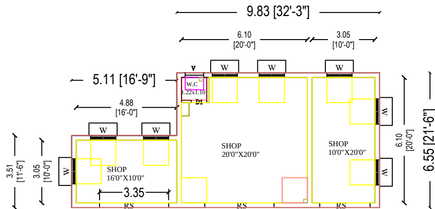
PROPOSED PLAN
