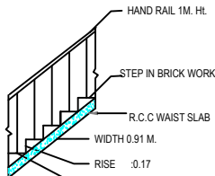
STAIR DETAIL
