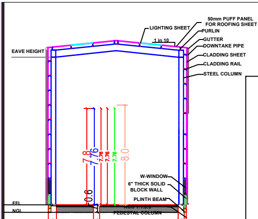
CROSS SECTIONAL ELEVATION
