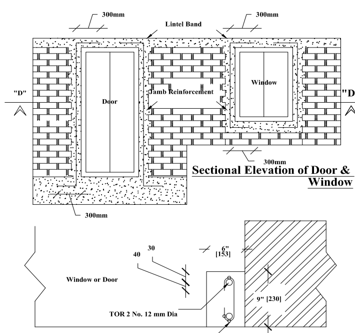
TYPICAL DETAILS OF PROVIDING VERTICAL STEEL BARS AROUND DOOR / WINDOWS
