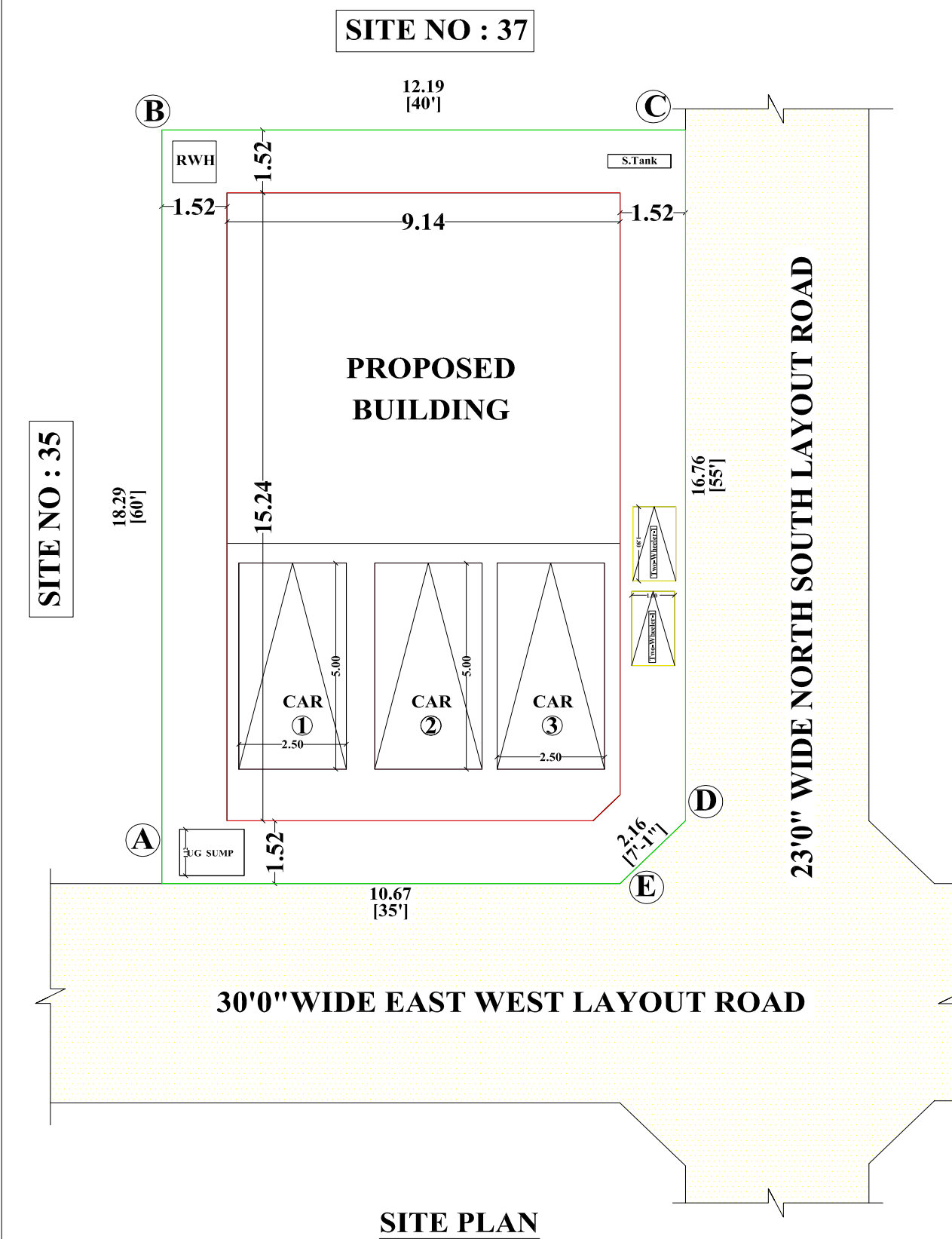
SITE PLAN
