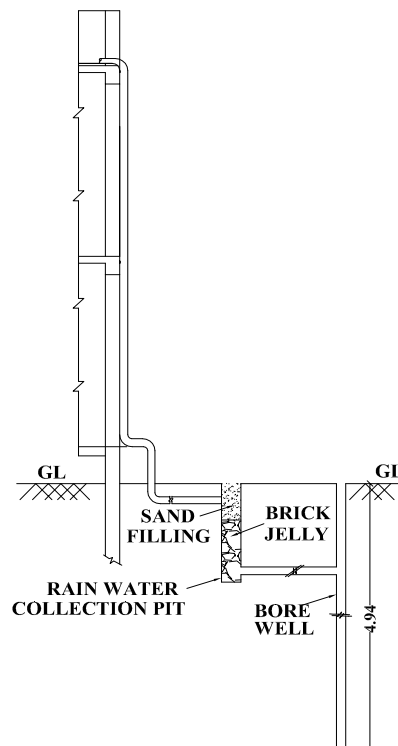
RAIN WATER HARVESTING SYSTEM
