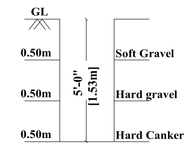
TRIAL-PIT
