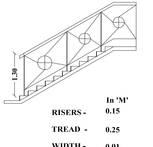
STAIR CASE DETAILS
