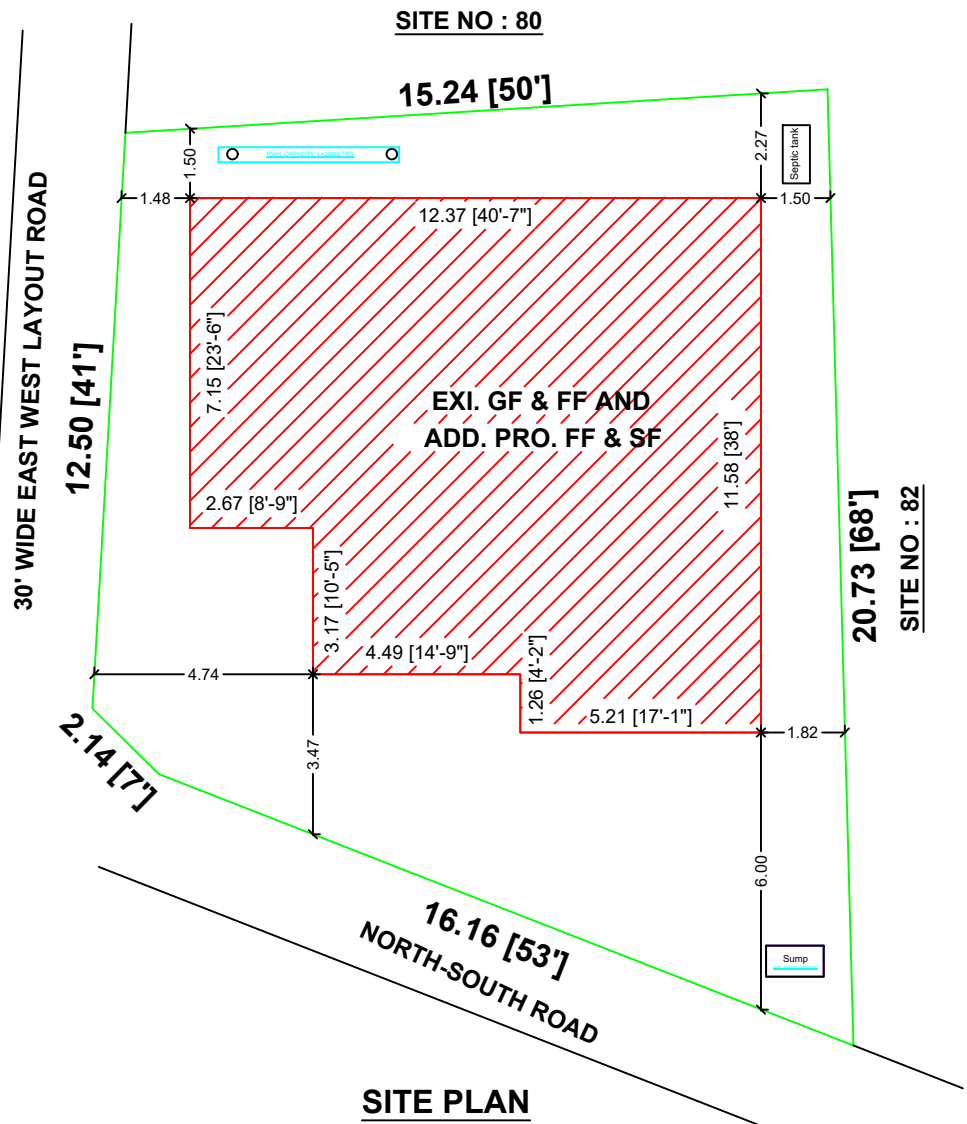
SITE PLAN
