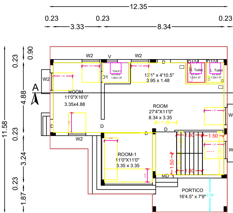
G FLOOR PLAN
