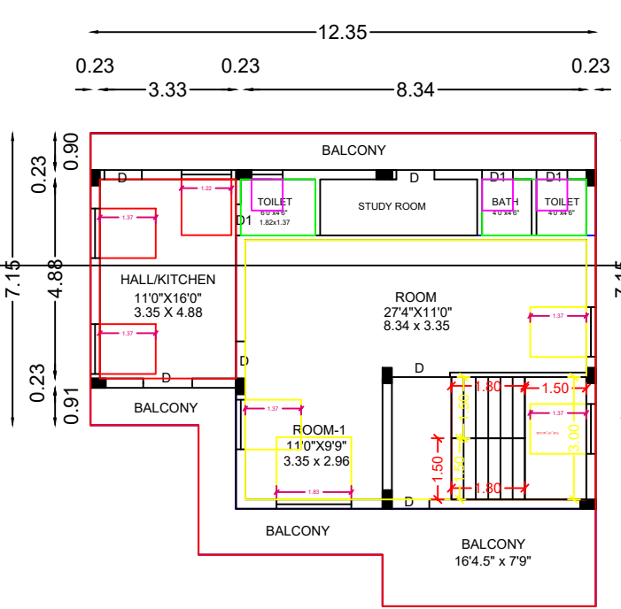
EXI. & ADD. PRO. FIRST FLOOR PLAN
