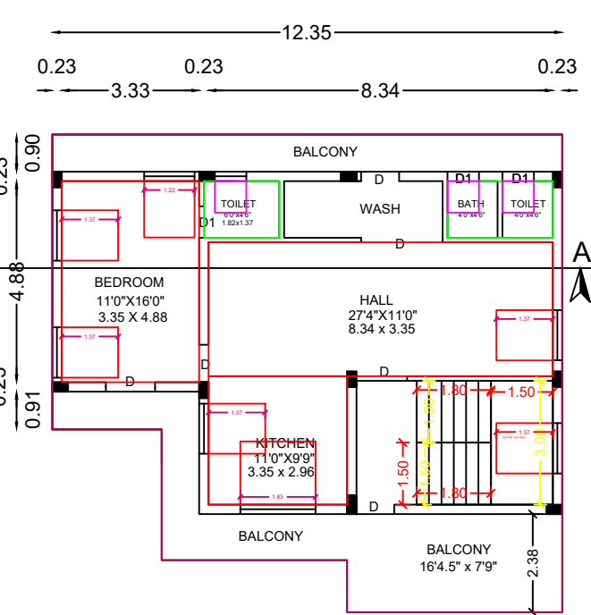
ADD. PRO. SECOND FLOOR PLAN
