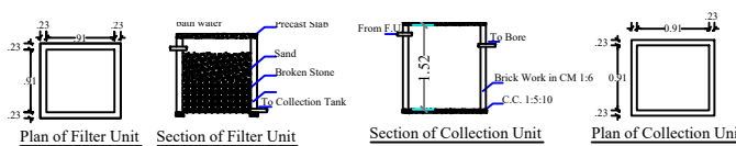
RAIN WATER PERCOLATION PIT
