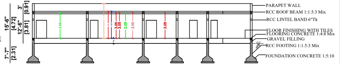
SECTION ON A-A SCALE 1:100
