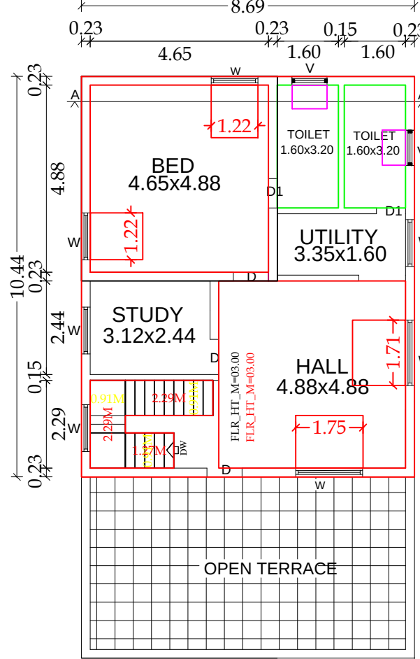
PRO. ADD. SECOND FLOOR
