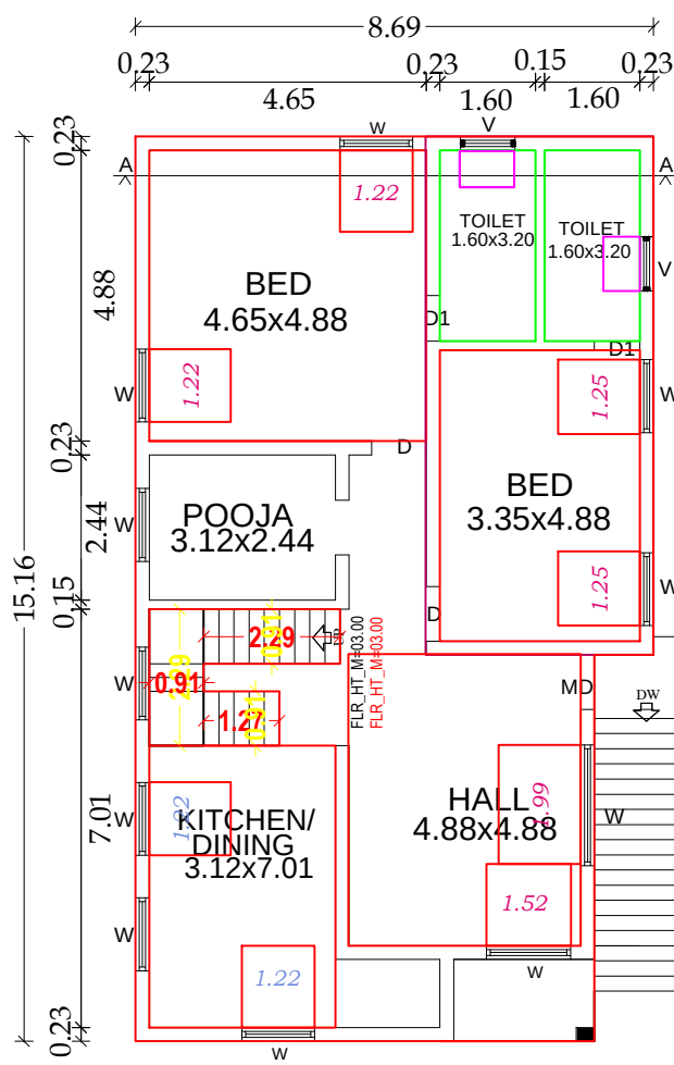
PRO. ADD. FIRST FLOOR
