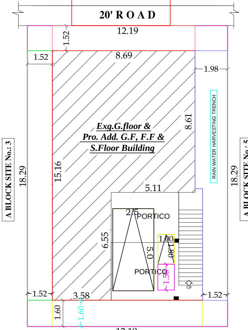
SITE PLAN
