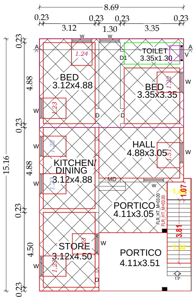
EXG. & PRO. ADD. GROUND FLOOR
