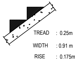
STAIRCASE DETAIL:
