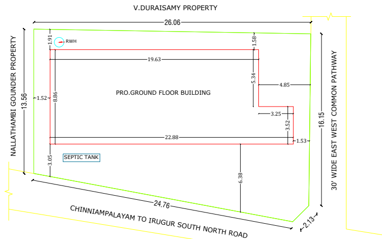
SITE PLAN
