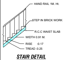
STAIR DETAIL
