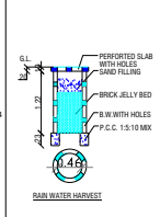
RAIN WATER HARVESTING
