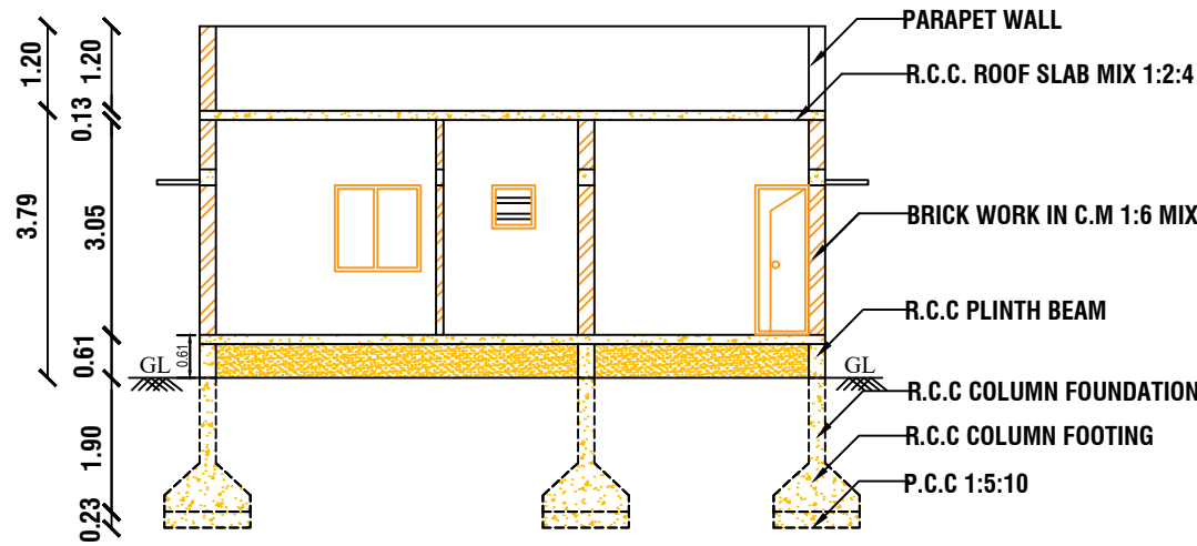
CROSS SECTION AT A-A
