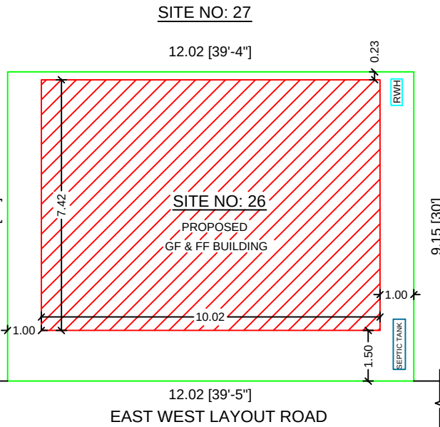
EAST WEST LAYOUT ROAD
