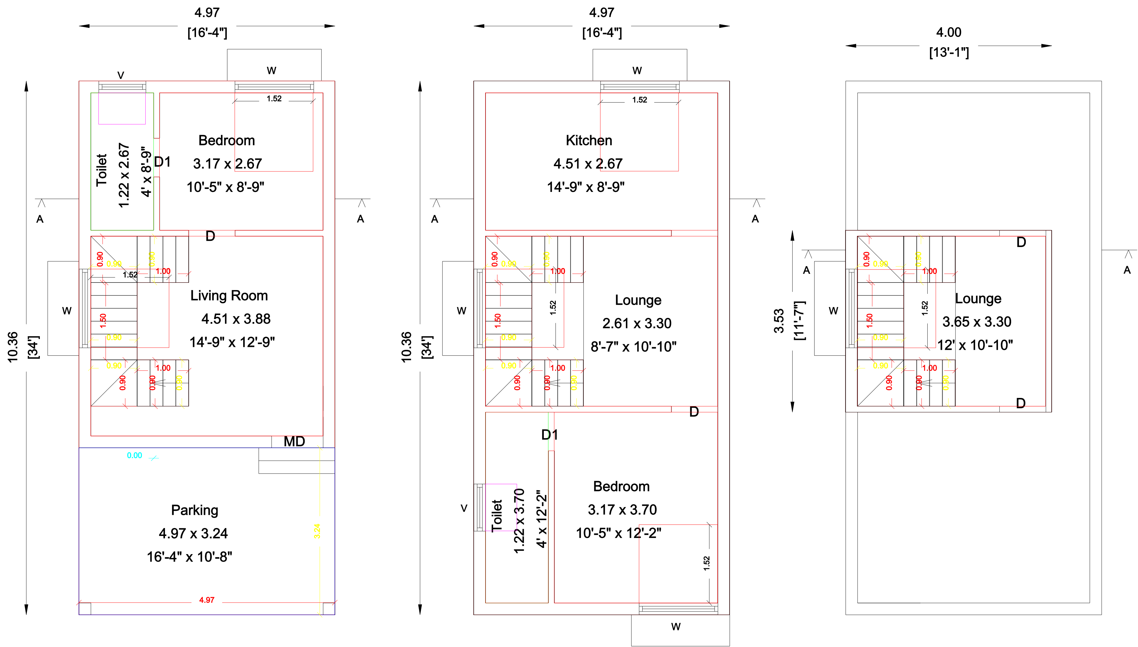
FLOOR PLAN
