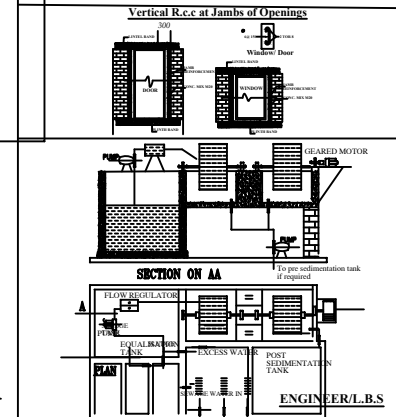
SEWAGE TREATMENT PLANT DETAILS (WASTE WATER RECYCLING UNIT)
