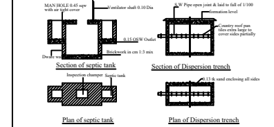
SEPTIC TANK
