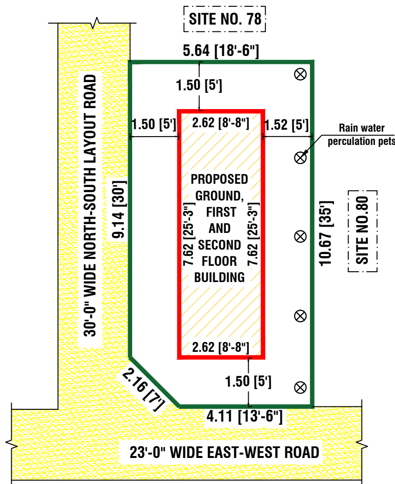
SITE PLAN
