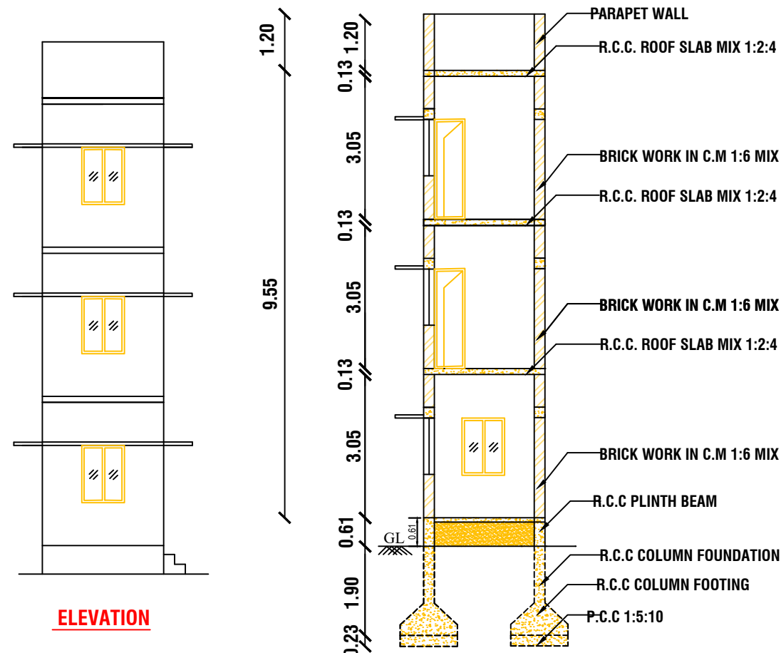
CROSS SECTION AT A-A
