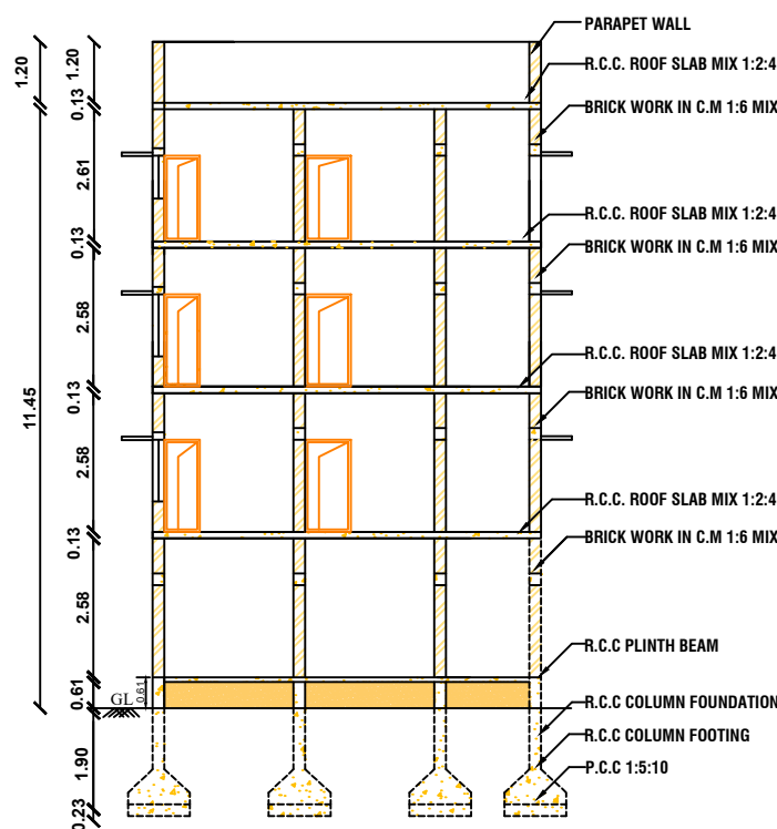
CROSS SECTION AT A-A
