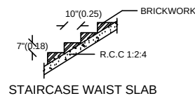
STAIRCASE WAIST SLAB
