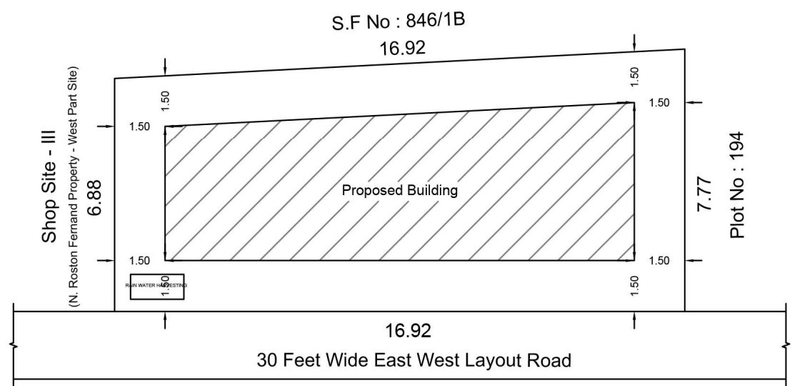
SITE PLAN
