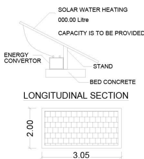
SOLAR SYSTEM
