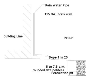
PERCOLATION PIT
