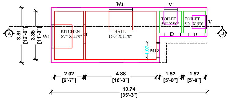
PROPOSED GROUND FLOOR PLAN BLOCK-2
