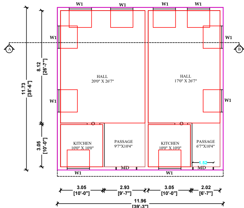
PROPOSED GROUND FLOOR PLAN BLOCK-1
