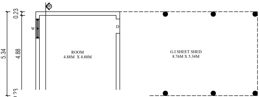
ND FLOOR PLAN
