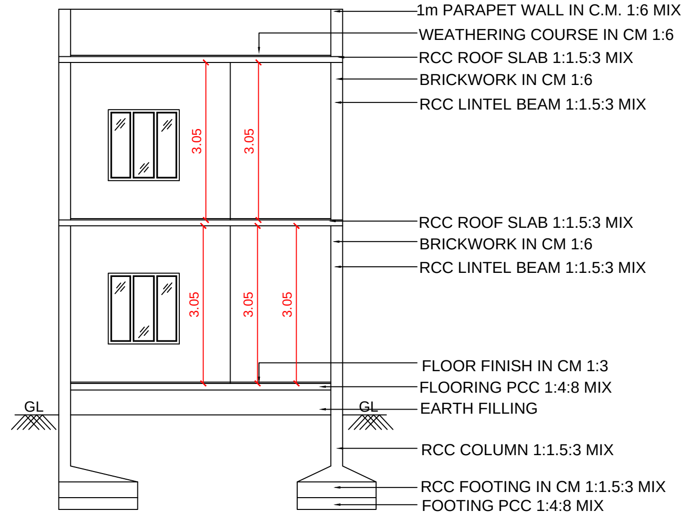
CROSS SECTION ON XY
