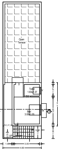
Pro. Second floor Plan Scale 1:100
