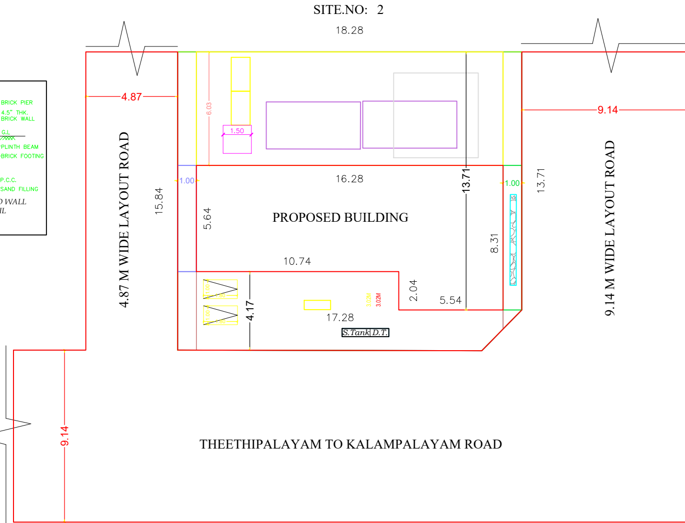
SITE PLAN
