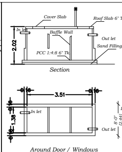
Sectional Elevation of Door and Window
