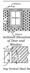
Section Around Door / Windows
