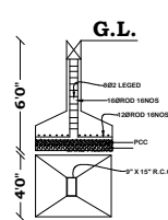
FOUNDATION DETAILS (NOT TO SCALE)
