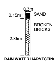
RAIN WATER HARVESTING DETAIL/PERCOLATION PIT (NTS)
