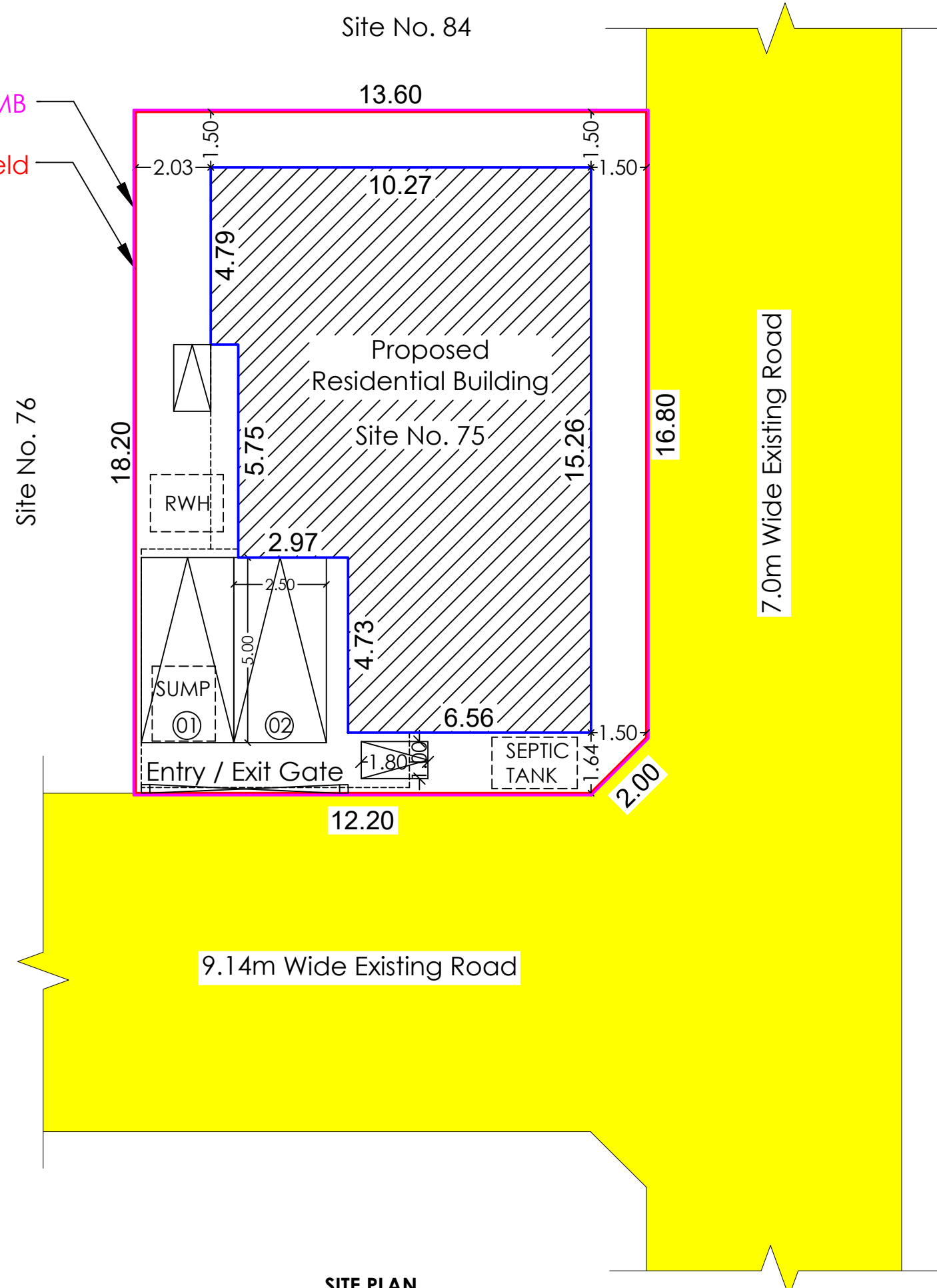
SITE PLAN
