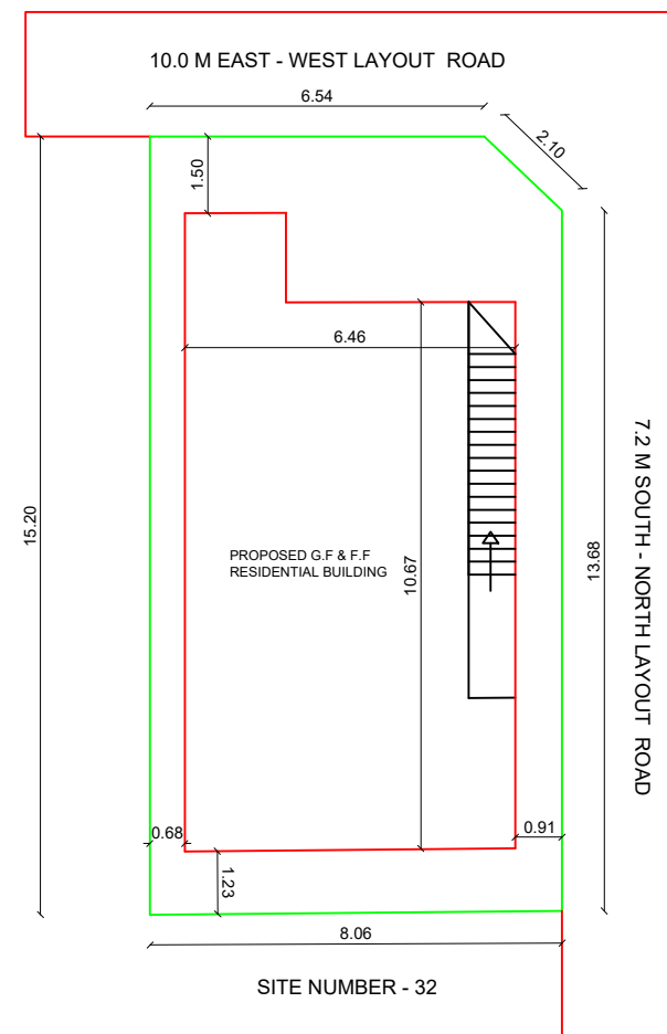
SITE PLAN
