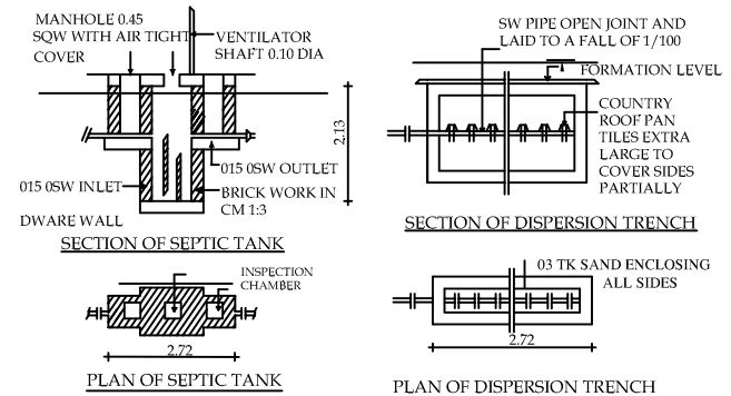
DETAILED DRAWING FOR SEPTIC TANK WITH DISPERSION TRENCH 125 GALLONS CAPACITY OF 1000 LITRES
