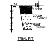
TRIAL PIT
