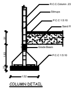
COLUMN DETAIL
