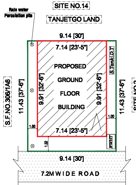
SITE PLAN
