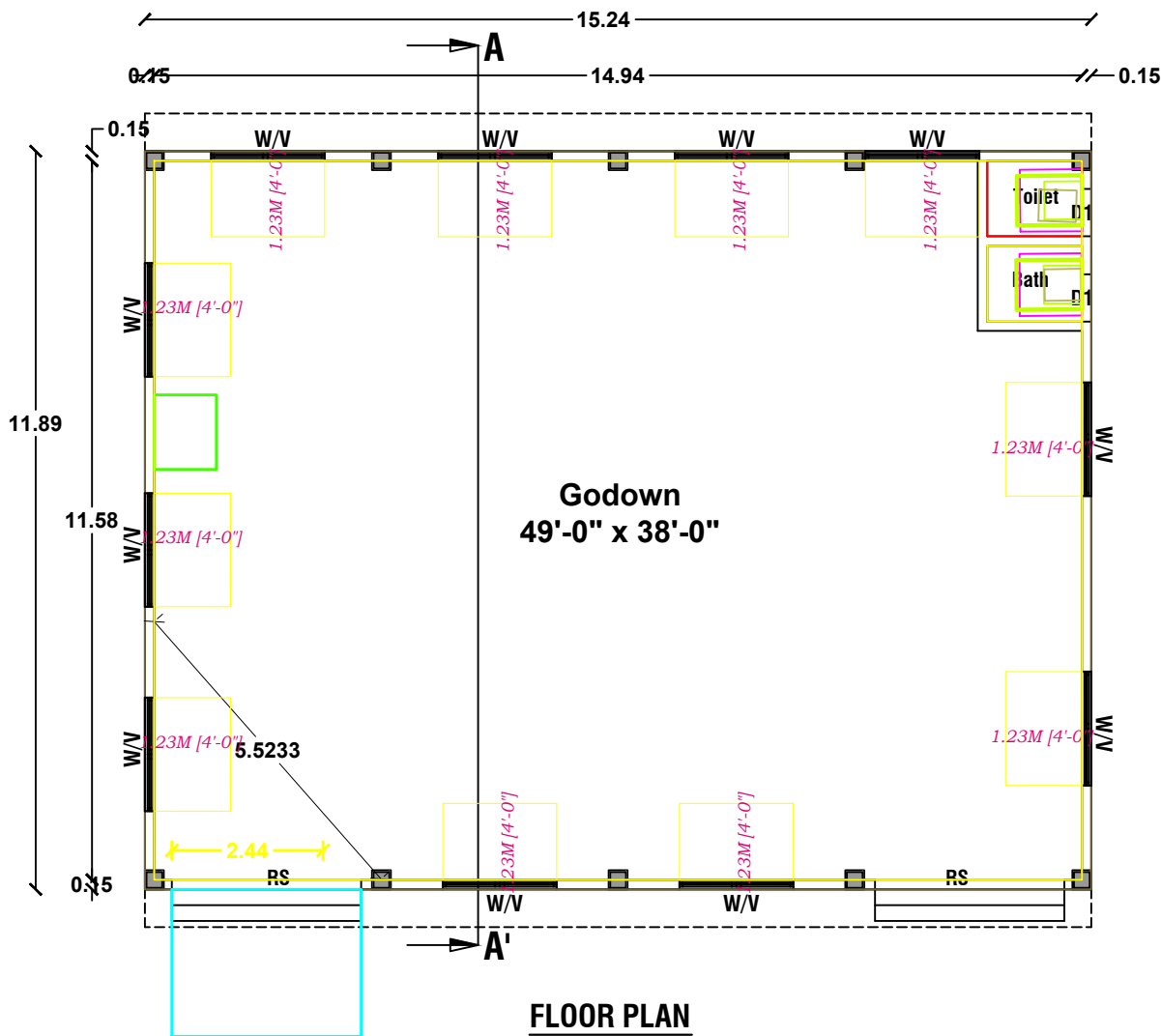
FLOOR PLAN
