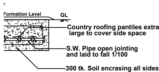
SEPTIC TANK WITH DISPERSION TRENCH ( 250 Gls.,)
