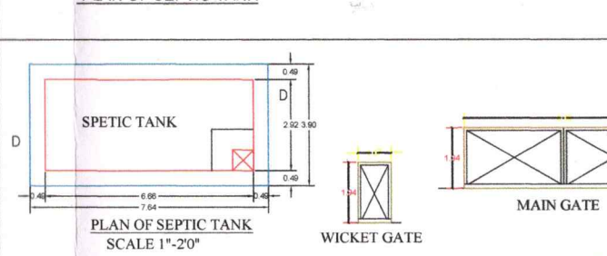
PLAN OF SEPTIC TANK SCALE 1"=20"
