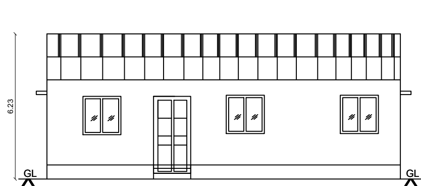
ELEVATION (WEST SIDE )
